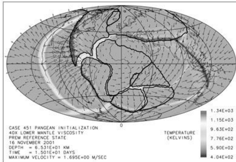
Figure 2(a). Snapshot of 3-D modeling solution after 15 days. The upper plot is an equal area projection of a spherical mantle surface 40 mi (65 km) below the earth's surface in which grayscale denotes absolute temperature. Arrows denote velocities in the plane of the cross-section. The dark lines denote plate boundaries where continental crust is present or boundaries between continent and ocean where both exist on the same plate. The lower plot is an equatorial cross-section in which the grayscale denotes temperature deviation from the average at a given depth.
